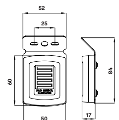
Rain Sensor
